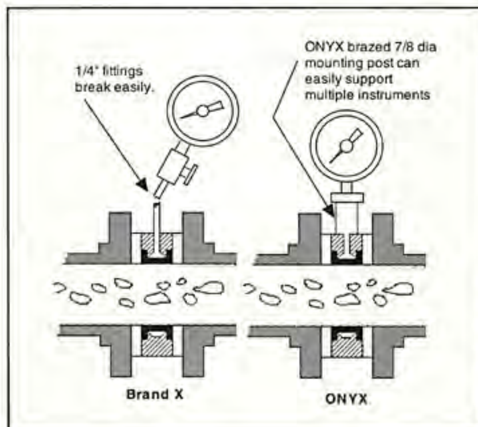
Robust 0.87" dia. mounting post resists breakage. Provides sturdy mounting for heavy gauges and instruments. Up to three gauges, pressure switches and transmitters can be combined on one isolator without additional support.
