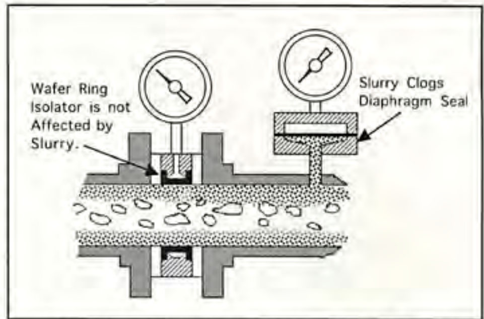
Diaphragm seal provides temporary solution, but stops working when slurry solidifies in the seal chamber.
