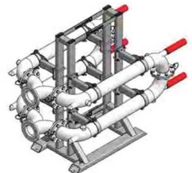
BioCrack 4 T-Pipe Assembly
